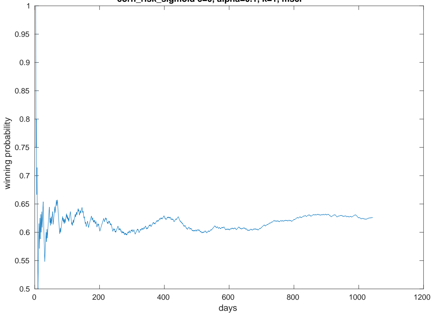
corn_risk_sigmoid c=0, alpha=0.1, k=1, msci
